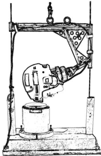
Front Impacts
